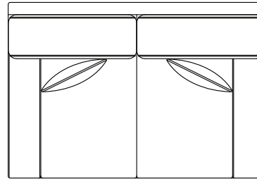
LOVESEAT 37"H x 63"W x 43"D •US636
